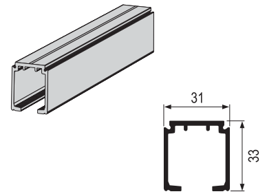
PVD TS-1280 gornja šina AL (PVS)
