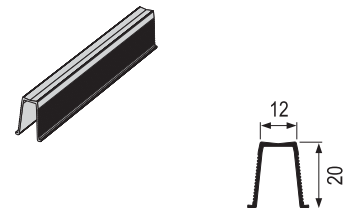
PVD PVC donja vodica TS
